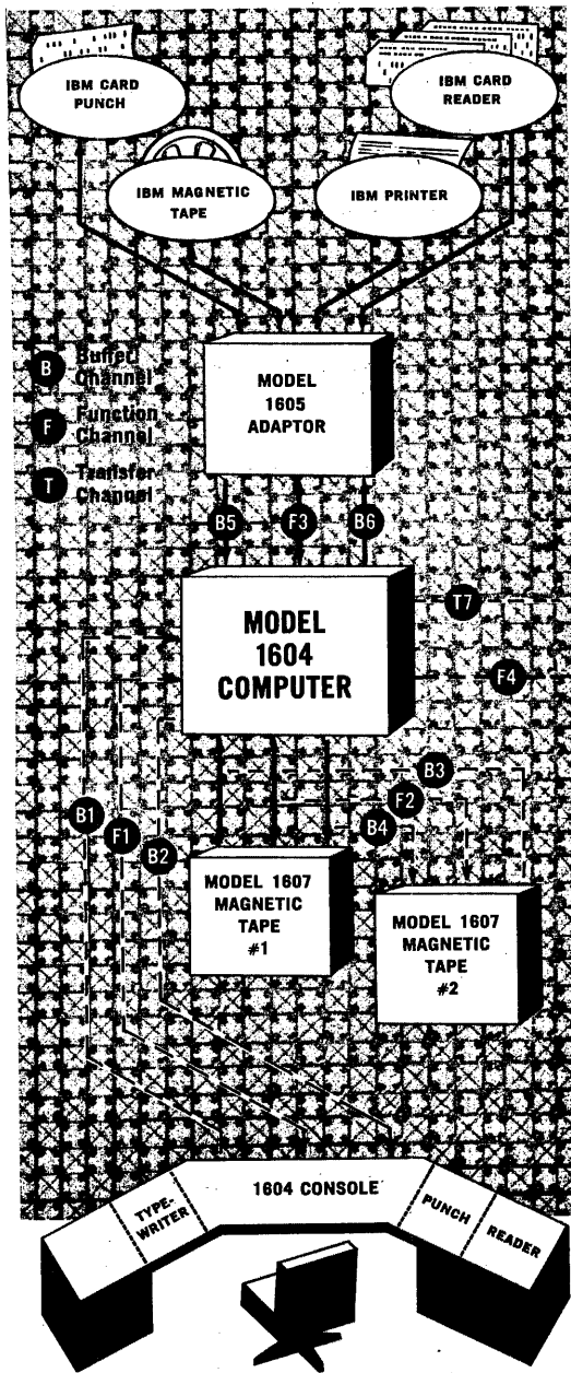
Diagram of Model 1604 Input-Output Facilities
